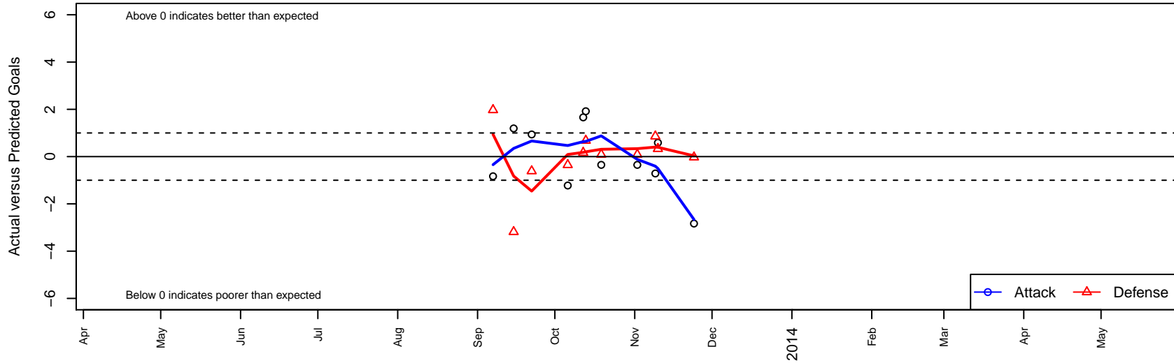
CA San Jose United B98 Dots are actual minus expected GF (blue circles) and GA (red triangles). Blue line is smoothed change in attack strength. Red is smoothed change in defense strength.
